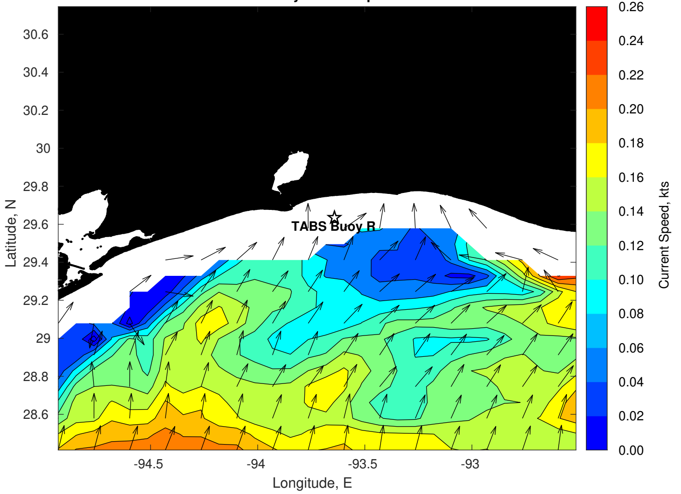
Surface Currents for TABS Buoy R at 04-Apr-2023 00:00:00
