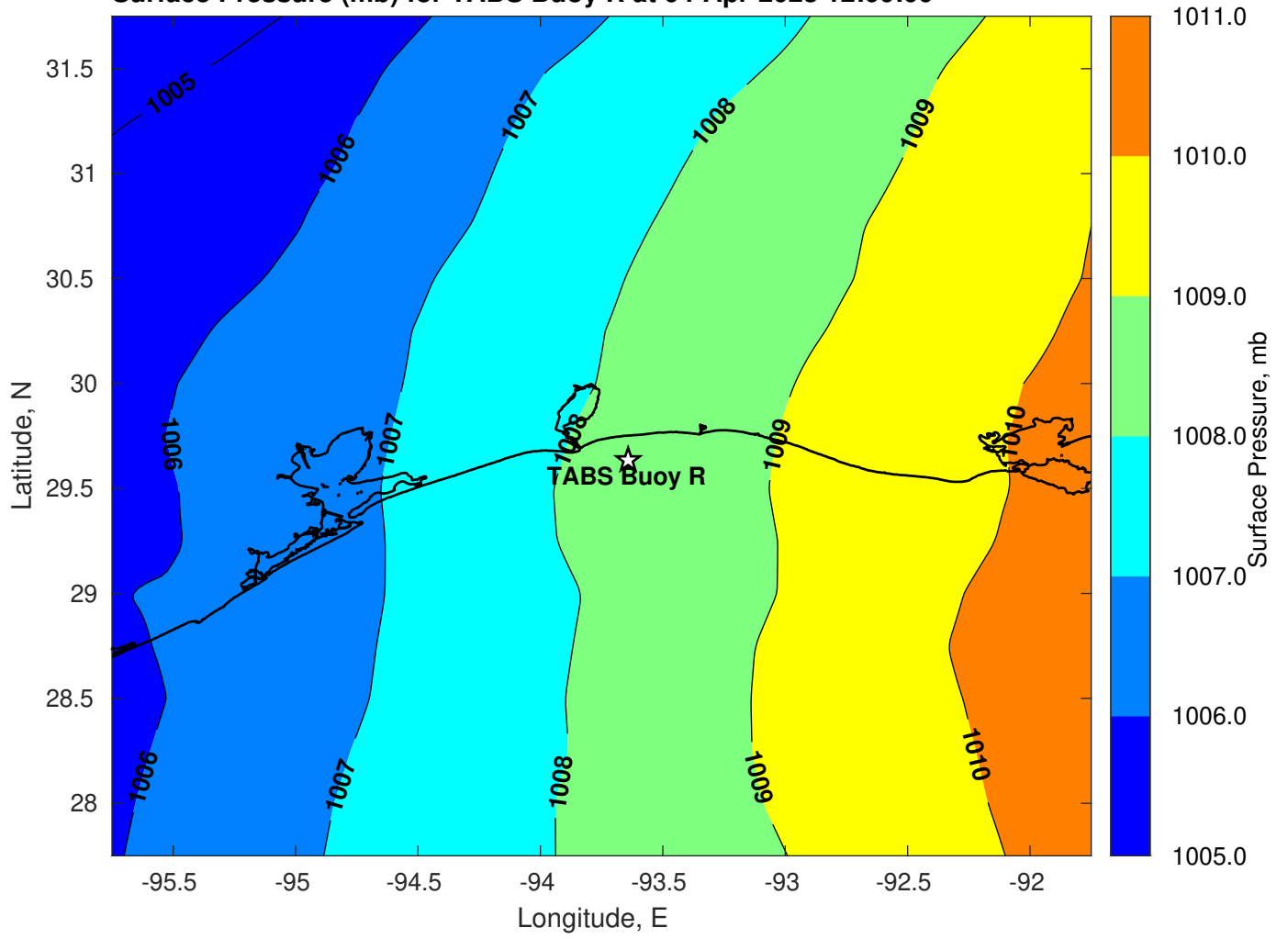
Surface Pressure (mb) for TABS Buoy R at 04-Apr-2023 12:00:00
